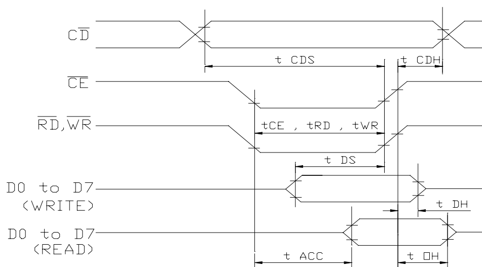
Bus Timing
